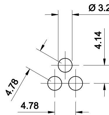
Enlarged Detail
