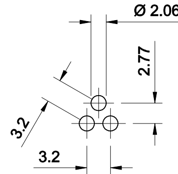
Enlarged Detail
